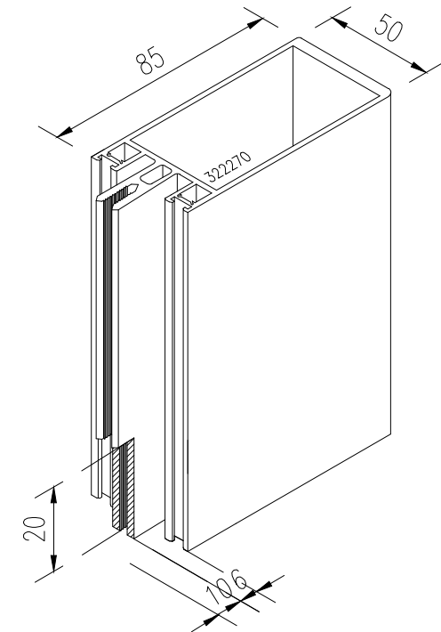
DETAIL -2
